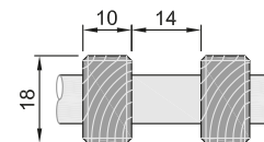
Grille - cross section
